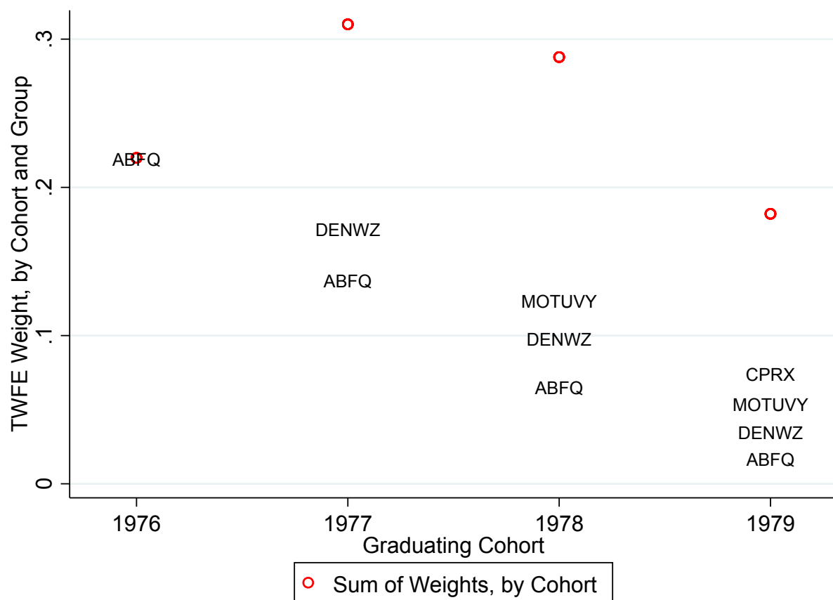
Appendix Figure A.4: TWFE Weights
