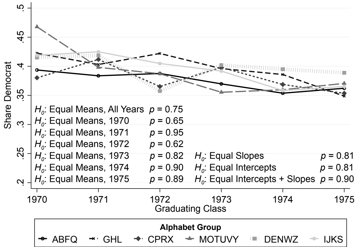
Appendix Figure A.3: Pretrends, by Alphabet Group
